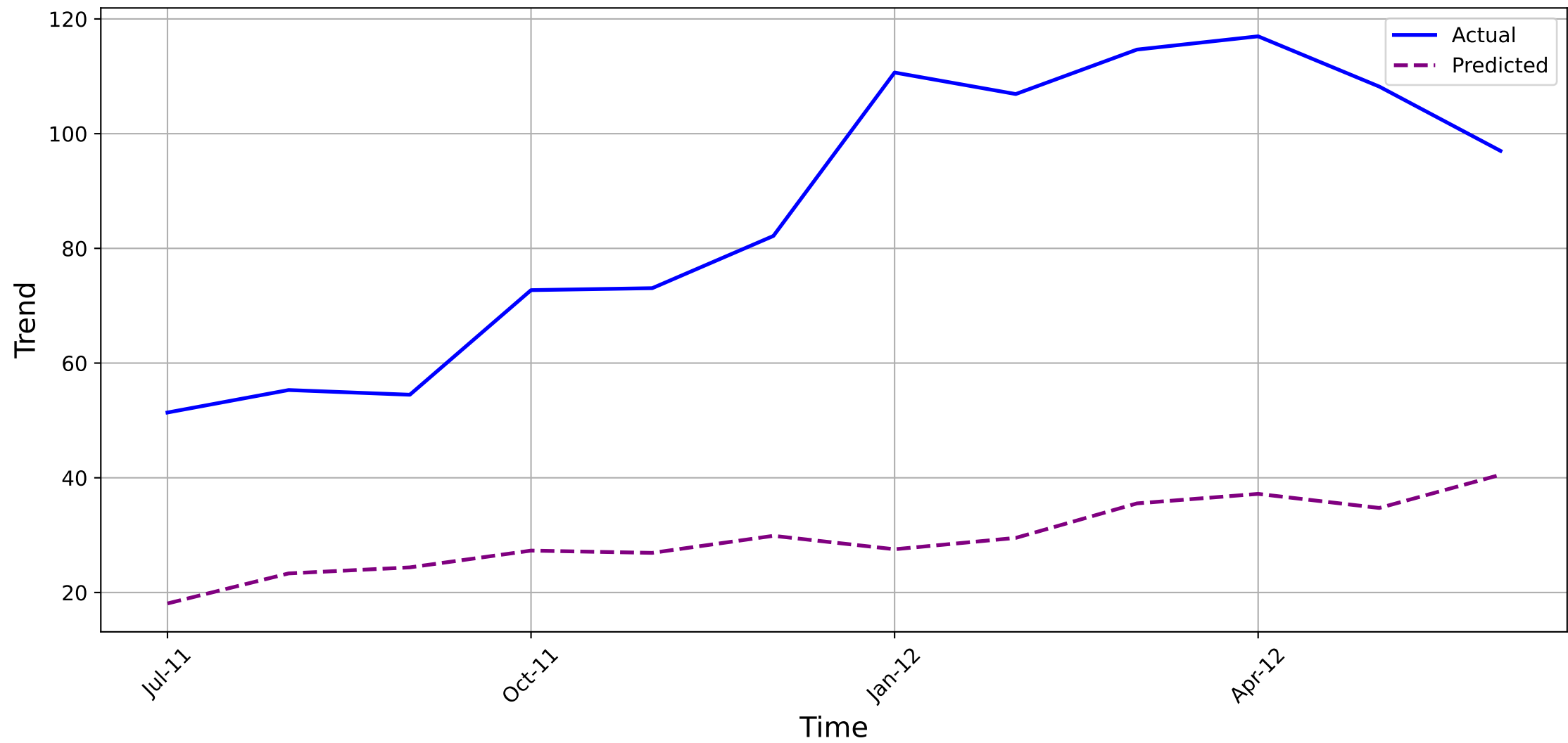
Password Attack-ALL - Validation
